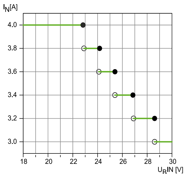
Fig. 5-2: Tripping current
