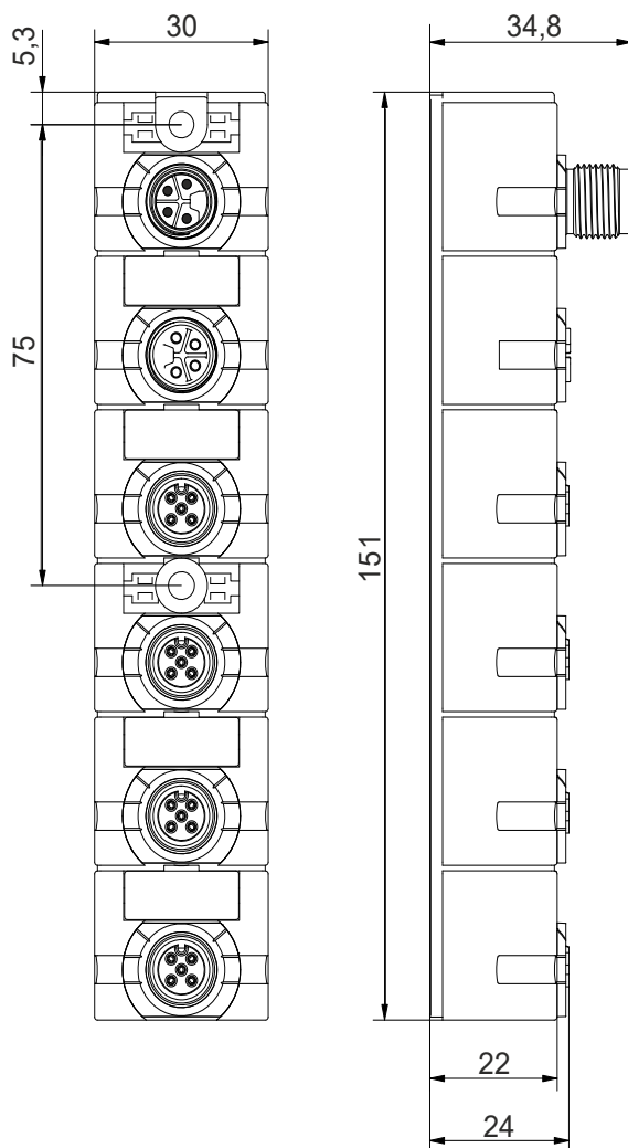
Fig. 6-1: Dimensions mm
