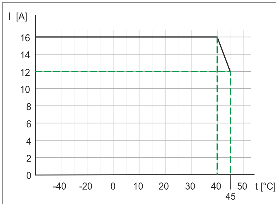
Fig. 3-1: Total current power output OUT pin 4 (pin 2)
